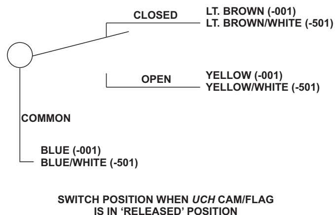
Figure 2. Microswitch in Released Position
